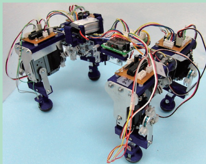
Quadruped robot driven by a fully decentralized control
