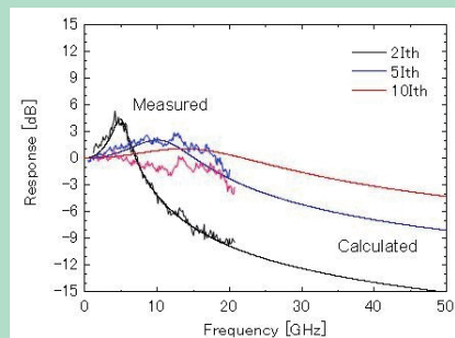
Measured and calculated response of functional semiconductor photonic device.
