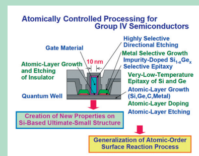
Atomically controlled processing for group IV semiconductors.
