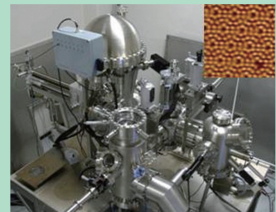
A UHV-compatible process/analyses system and the STM image of a Si surface (inset).
