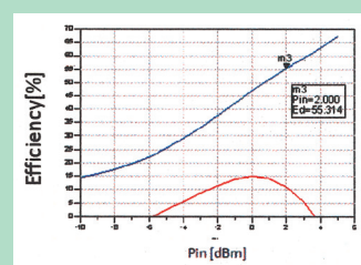
Fig. 3 Drain efficiency of 60 GHz source ground PA
