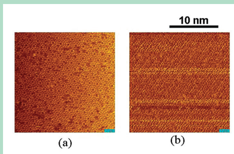
S(111) 7X7 atomic structure taken by SNDM. (a)Topography (b) Electric dipole-moment.
