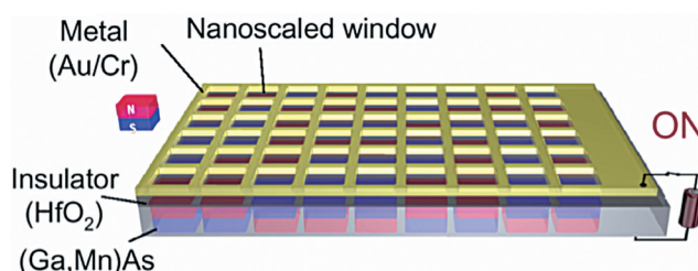
(Left) Schematic of electric-field defined magnetic nano-dots. (Right) Development of the world's first high performance 40 nm \phi magnetic tunnel junctions (MTJs) with CoFeB/MgO perpendicular anisotropy.
