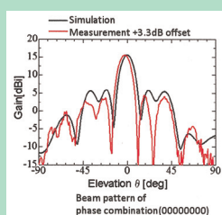
Fig. 1 Double slot beam forming antenna (top) and its directivity (bottom)
