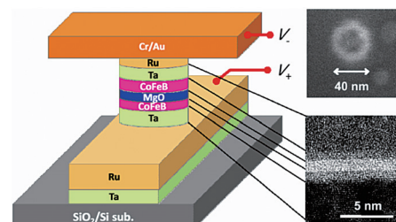
(Left) Schematic of electric-field defined magnetic nano-dots. (Right) Development of the world's first high performance 40 nm \phi magnetic tunnel junctions (MTJs) with CoFeB/MgO perpendicular anisotropy.
