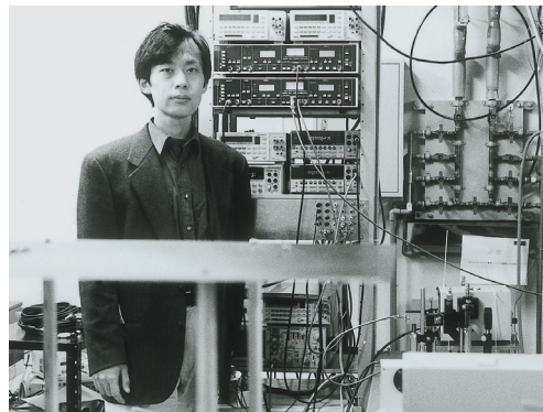
Semiconductor Spintronics
