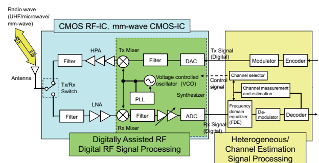
Fig.2 One-chip transceiver LSI for broadband wireless communication
