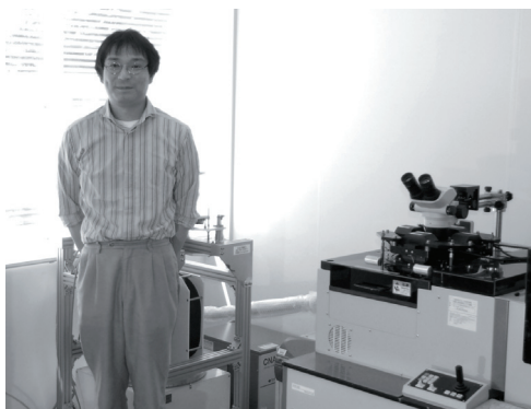
Semiconductor Spintronics
