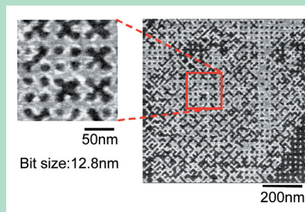
Example of a ferroelectric actual information storage (4 Tbit/inch 2 ).
