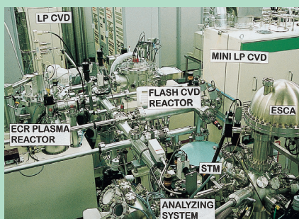
Atomically controlled processing systems for group IV semiconductors
