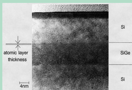
Atomic lattice image of a SiGe heterostructure grown by CVD at 500°C.
