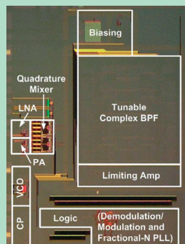
Transceiver IC for Sensor Network Systems
