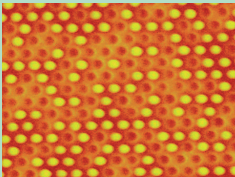
MFM images of a L1,-CoPt patterned films (One of fundamental technologies to realize densities of over 2 Tbits/in 2 .)
