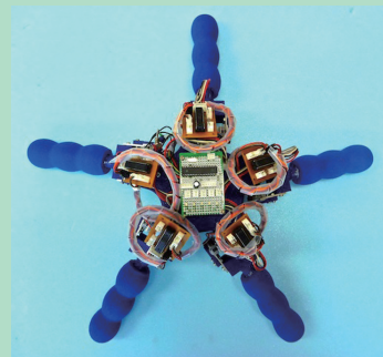
Ophiroid robot that enables omnidirectional locomotion
