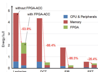
Nonvolatile FPGA for energy-efficient MCU
