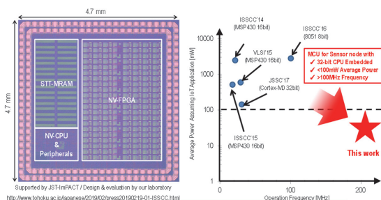
Nonvolatile microcontroller unit
