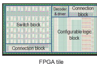
FPGA tile
