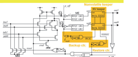
Ultra-low power dark-silicon circuits
