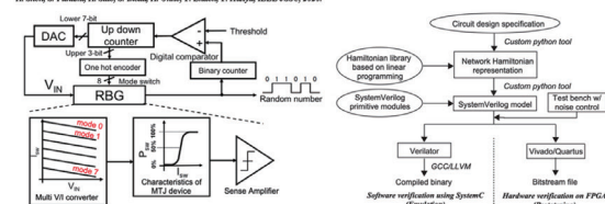
High-throughput/low-energy TRNG
