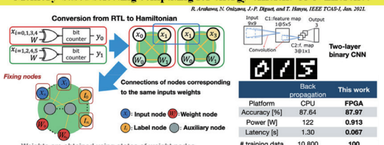
Energy-efficient BCNN inference hardware based on CMOS invertible logic
