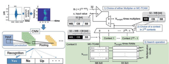
Memory-based selecting computing for energy-efficient CNN inference
