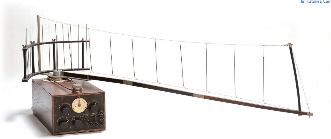
八木・宇田アンテナの実験装置 (1929) Experimental equipment for Yagi-Uda Antenna (1929)
