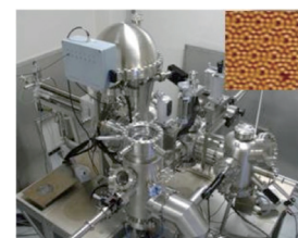
図3. 超高真空プロセス・評価一貫装置とSi表面のSTM像(右上) Fig3. A UHV-compatible process/analyses system and the STM image of a Si surface (inset).
