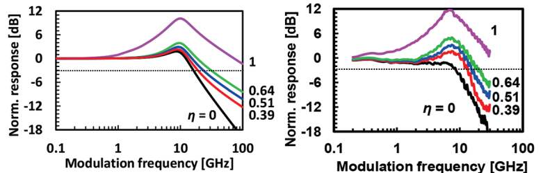
レーザ周波数応答特性の計算結果(左図)と試作素子による測定結果(右図) Frequency response of the laser; simulated results (left) and measured result by using fabricated device (right)
