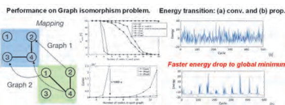
Fast solving larger combinatorial optimization problem than QA
