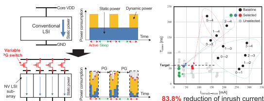
Operation-condition-aware power-gating-switch configuration
