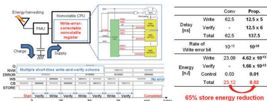
Error-Tolerant Nonvolatile Register for Energy-Aware Intermittent Computing K. Sakai, et al., IEEE MWSCAS, 2023.
