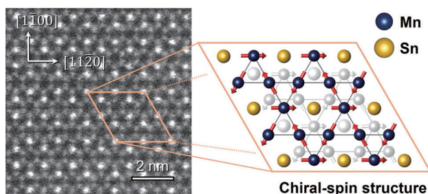
磁気八極子の特異な電流応答を解明したノンコリニア反強磁性 Mn 3 Sn 薄膜の断面 TEM 像 Cross-sectional TEM image of noncollinear-antiferromagnetic Mn 3 Sn film where unconventional physics of magnetic octupole dynamics is revealed
