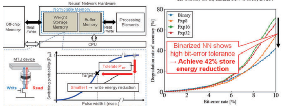
Write-Energy Reduction of MTJ-Based Quantized Neural-Network Hardware K. Asano, et al., IEEE ISMVL, 2023.
