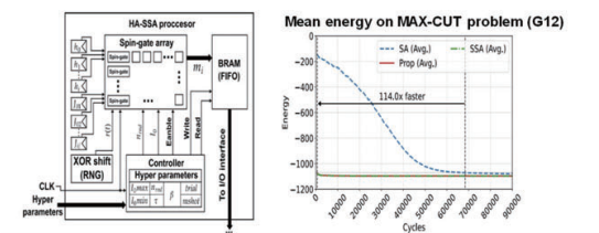
6-times memory efficient FPGA implementation with 2-times faster annealing D. Shin, et al., IEEE JETCAS, Mar. 2023.
