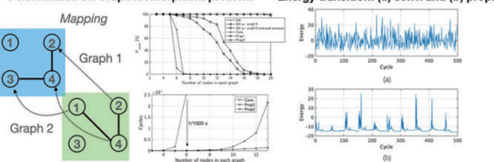
Fast solving larger combinatorial optimization problem than QA N. Onizawa, et al., IEEE TNNLS (to appear)
