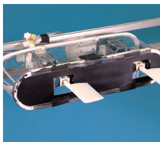
図 2. 生物規範制御に基づく古生物の運動復元 Fig.2 Reconstruction of extinct animal's locomotor patterns based on bio-inspired control mechanism
