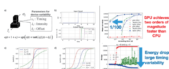
GPU-accelerated simulated annealing with p-bit device variability modeling
