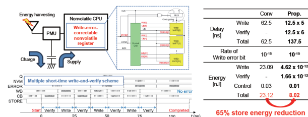
Nonvolatile Register with a Switching-Probability-Aware Store-and-Verify Scheme
